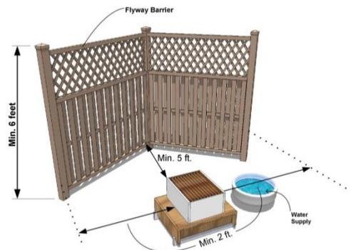
Example hive and flyway barrier, also see 17.4.3.F in Zoning Ordinance
